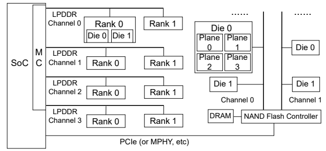
Fig. 2: Memory and storage systems on consumer devices.
